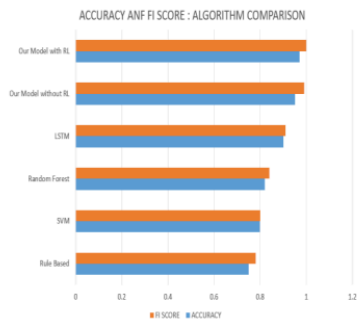
Chart 1. Algorithm Performance Comparison (with and without Reinforcement Learning)
